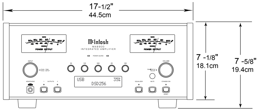
Front View of the MA8900
