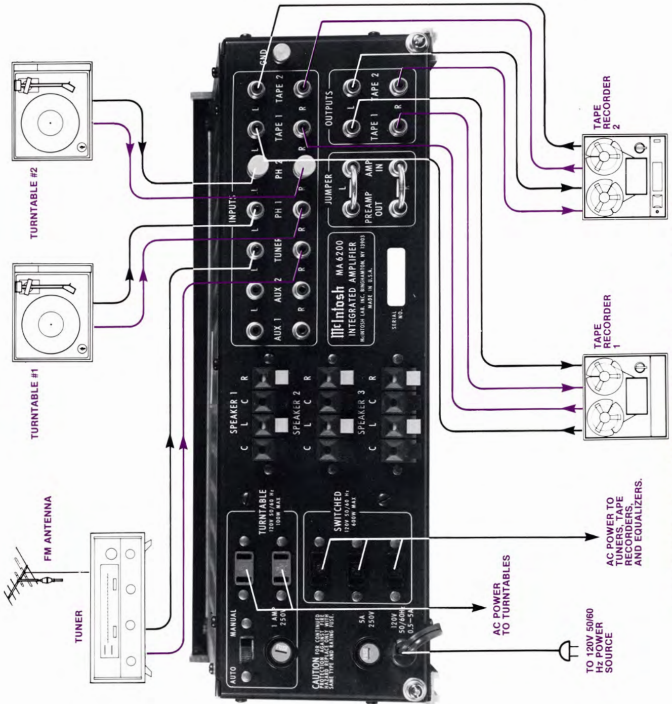
CONNECTIONS FOR TUNERS, TURNTABLES, AND TAPE RECORDERS
